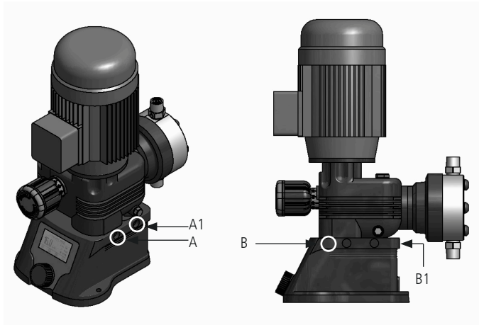
Fig. 6. Default to alternative position: move screws from A to A1 and from B to B1.
