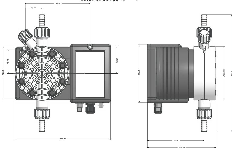
Corps de pompe "S" - "T"
