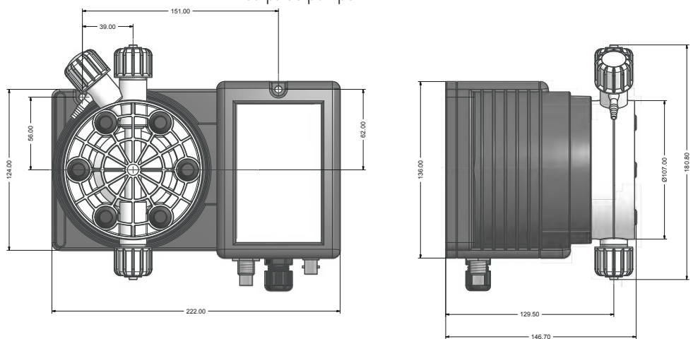
Corps de pompe "N" - "P"
